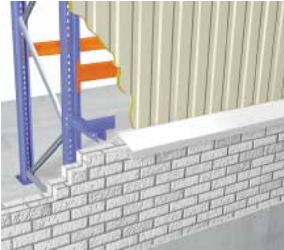
Roof and Side Cladding Section
