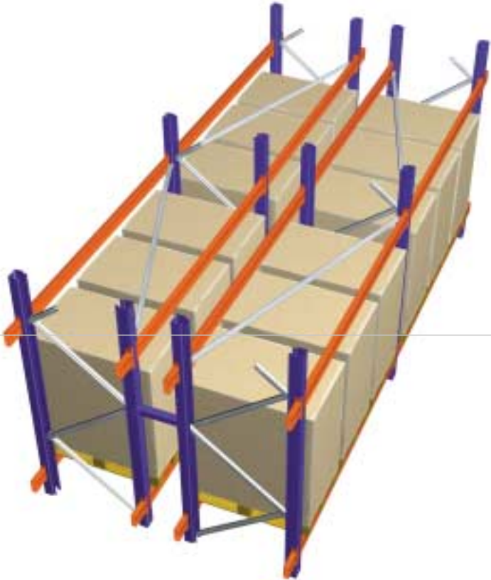
Horizontal Bracing
